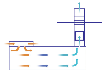
Modified Downdraft booth air flow
